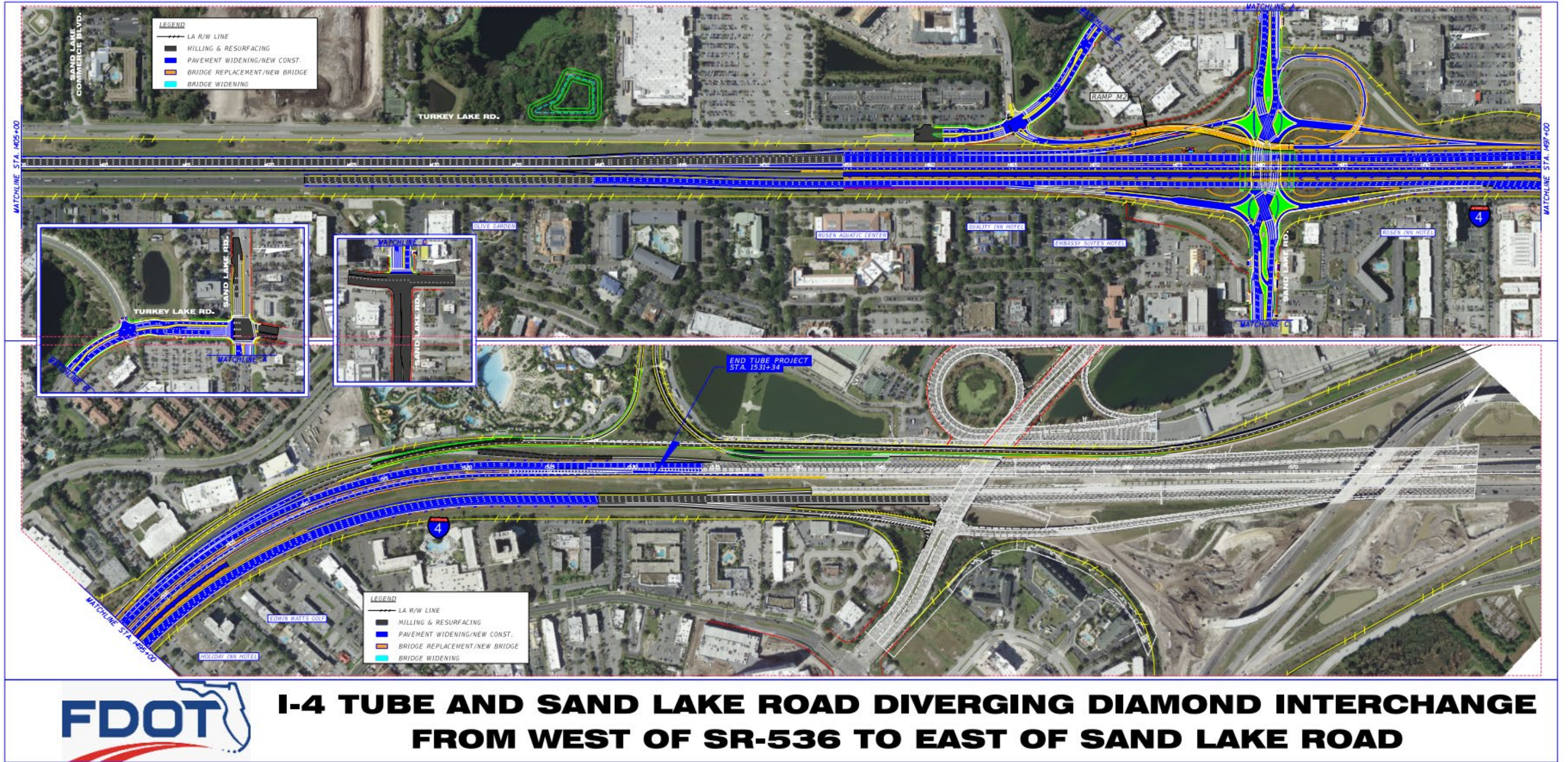
Figure 2: I-4 at Sand Lake Road – Design Exhibit
